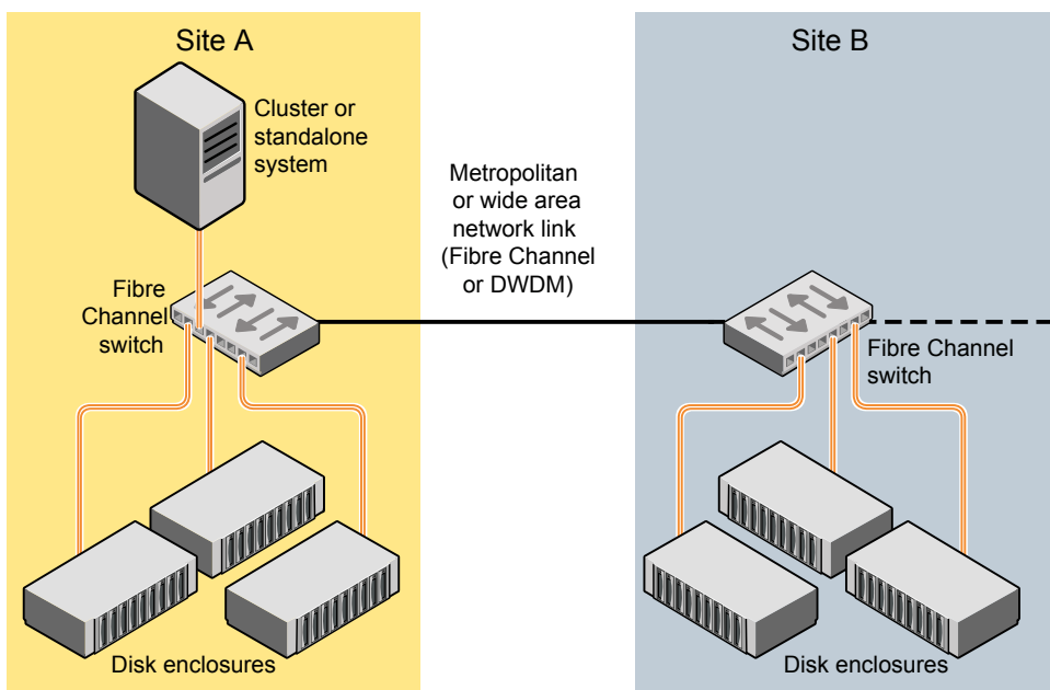
Figure 18-3 Example of a two-site configuration with remote storage only
