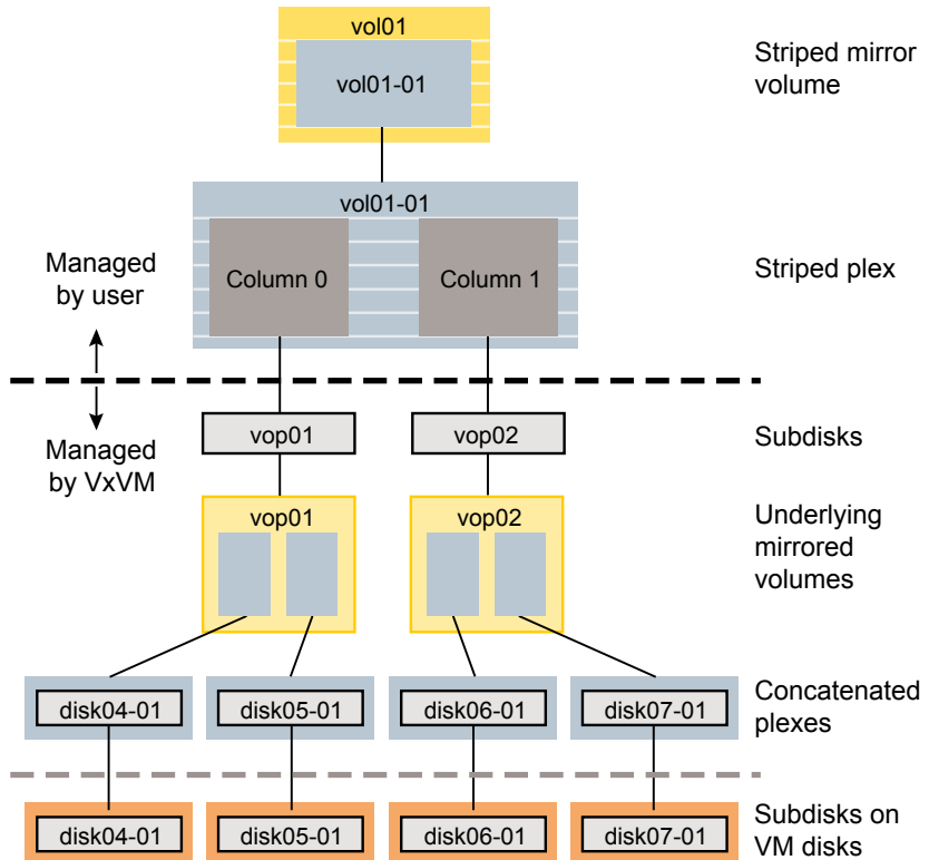
Figure 3-17 Example of a striped-mirror layered volume
