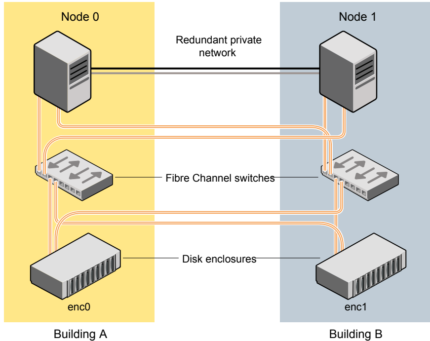
Figure 38-5 Typical arrangement of a 2-node campus cluster
