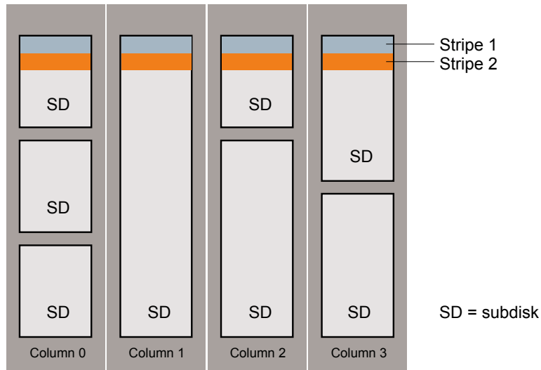
Figure 3-14 Veritas Volume Manager RAID-5 array
