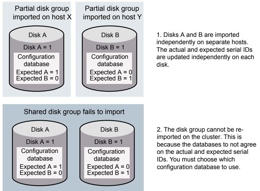
Figure 38-7 Example of a true serial split brain condition that cannot be resolved automatically
