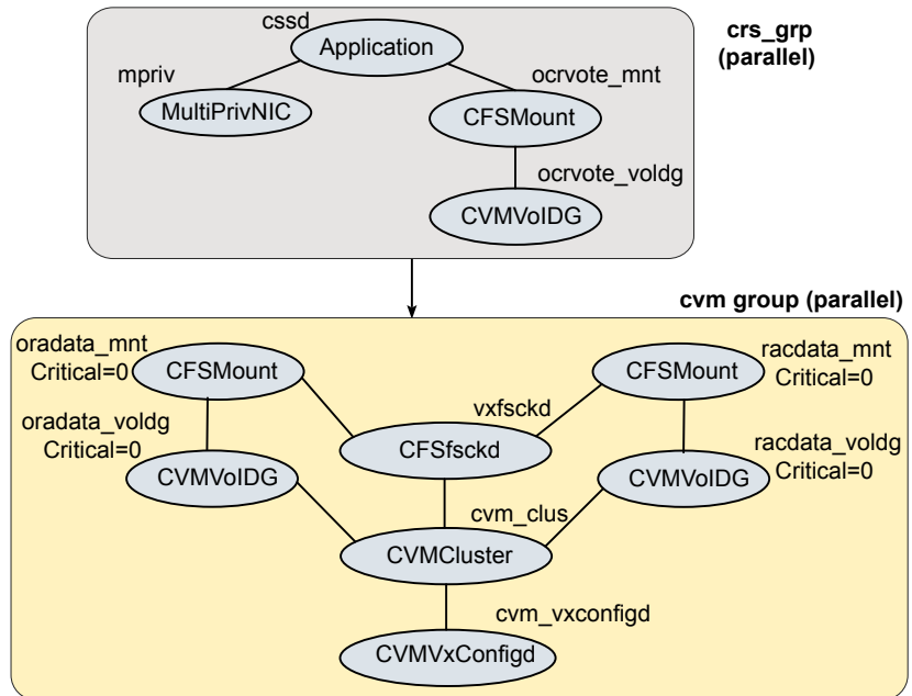
Figure 16-6 Service group configuration without the VCS Oracle agent (multiple databases)
