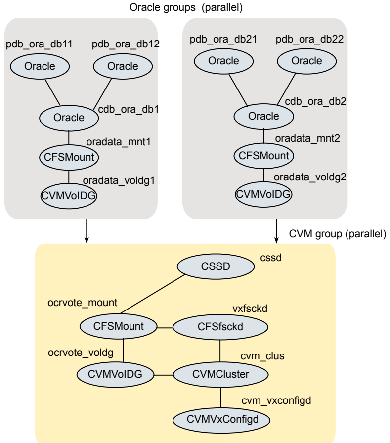
Figure 16-4 illustrates an alternate service group configuration with the VCS Oracle agent.
