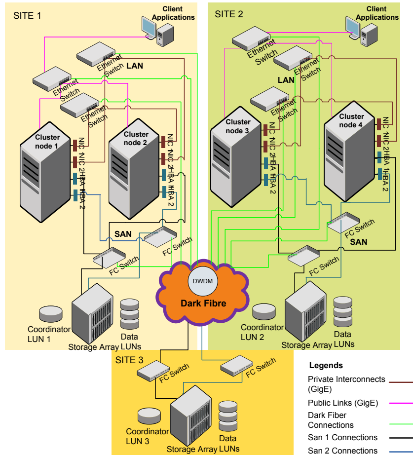
Figure 20-1 Sample SF Oracle RAC configuration
