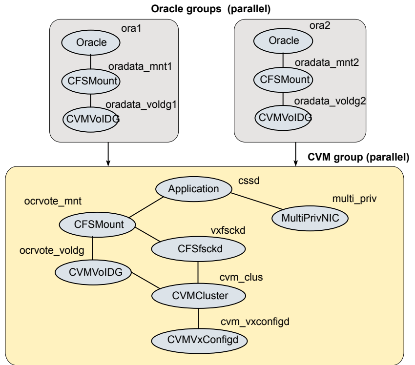
Figure 16-2 Service group configuration with the VCS Oracle agent
