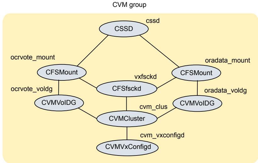
Figure 16-5 Service group configuration without VCS Oracle agent (single database)
