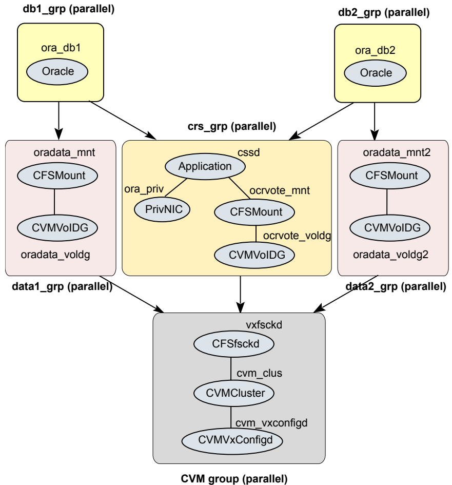
Figure 16-4 Service group configuration with the VCS Oracle agent (alternate configuration)
