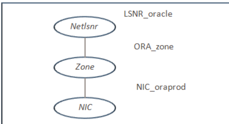
Figure B-10 Dependency for Netlsnr service group
