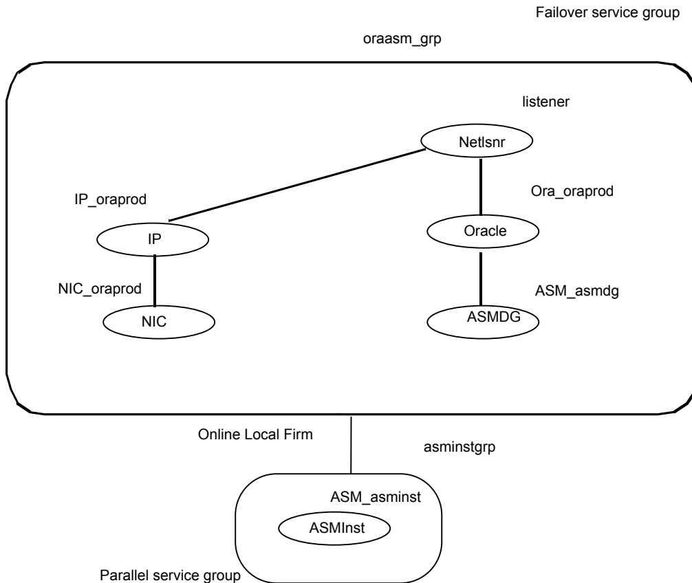
Figure B-17 Dependency graph with ASMIInst resource as a parallel service group
