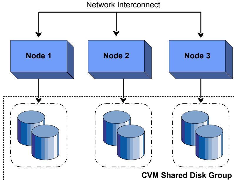
Figure 6-11 Flexible Storage Sharing Environment
