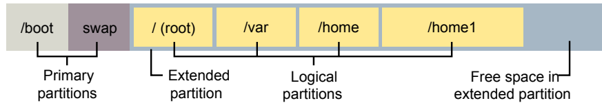
Figure 42-3 Boot and swap configured on two primary partitions, and free space in the extended partition
