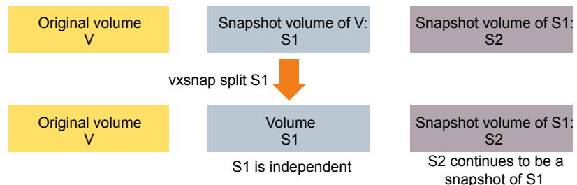
Figure 17-7 Splitting snapshots
