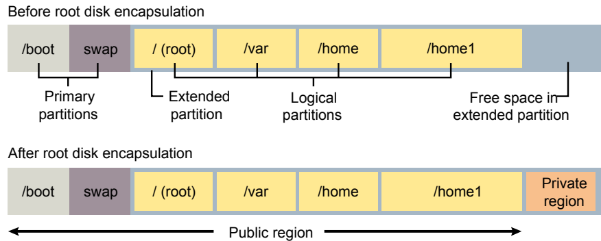
Figure 43-3 Boot and swap configured on two primary partitions, and free space in the extended partition
