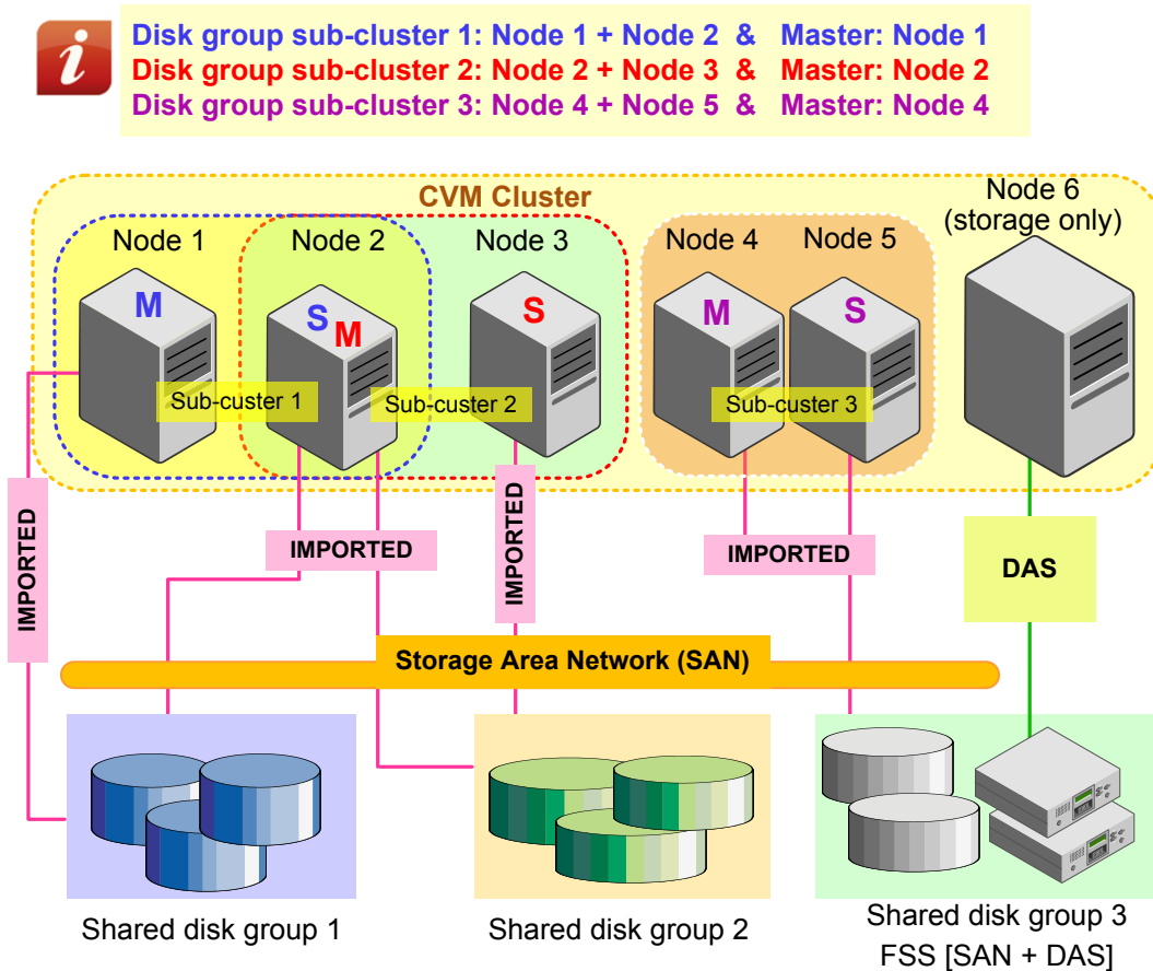
Figure 6-12 Disk group sub-clustering for the application isolation feature
