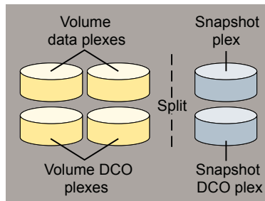
Figure 42-4 Examples of disk groups that can and cannot be split
