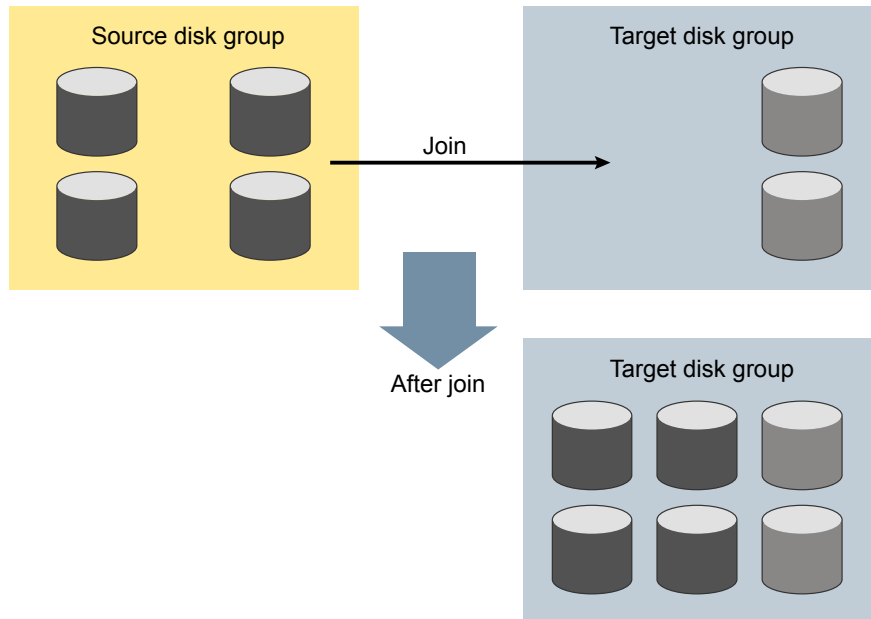
Figure 42-3 Disk group join operation
