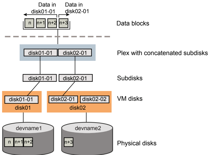
Figure 3-6 Example of spanning
