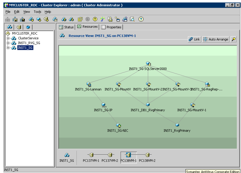
Figure 5-9 Typical SQL Server 2000 service group RDC configuration
