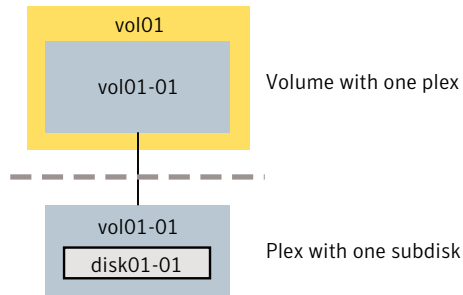
Figure 1-10 Example of a volume with one plex
