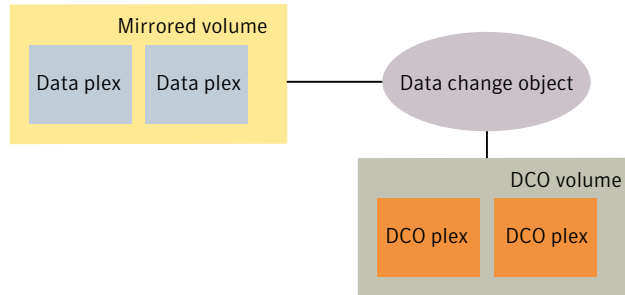
Figure 1-32 Mirrored volume with persistent FastResync enabled
