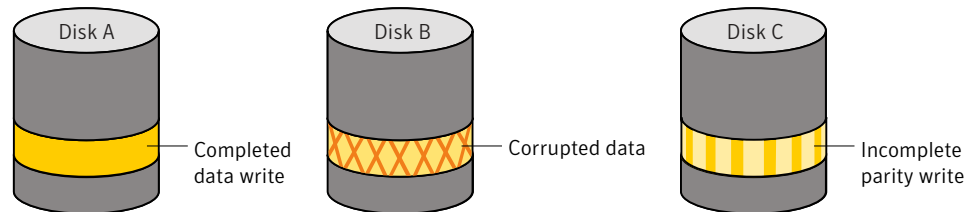
Figure 1-24 Incomplete write to a RAID-5 volume
