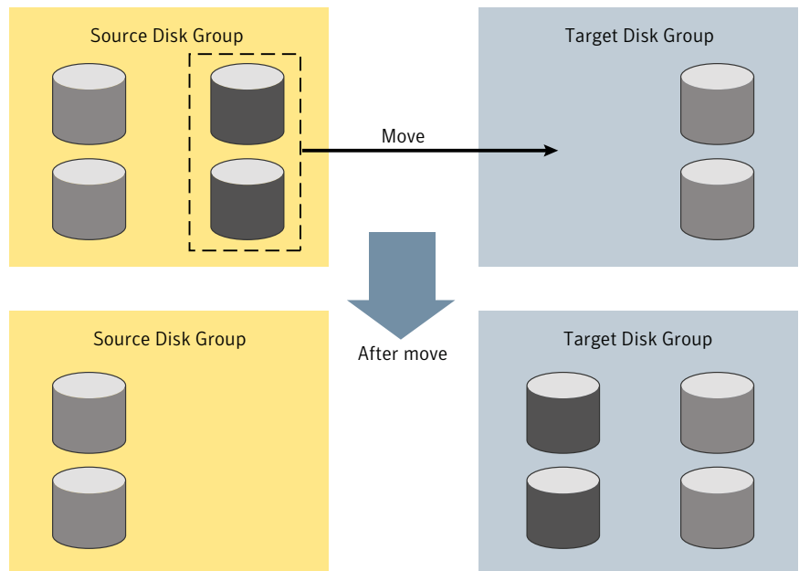
Figure 4-4 Disk group move operation
