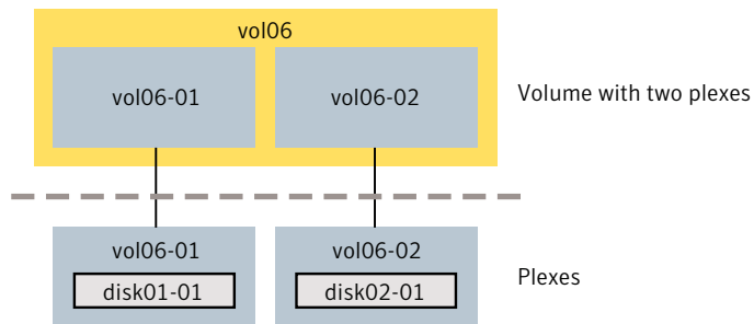
Figure 1-11 Example of a volume with two plexes
