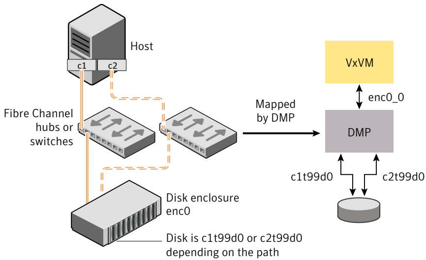
Figure 3-2 Example of multipathing for a disk enclosure in a SAN environment
