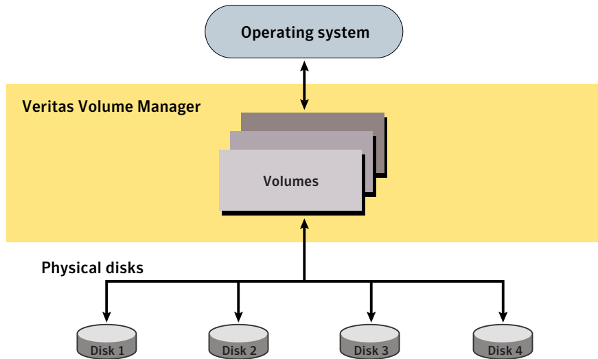
Figure 1-2 How VxVM presents the disks in a disk array as volumes to the operating system
