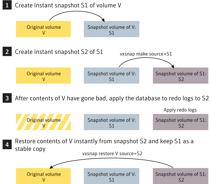
Figure 9-6 Using a snapshot of a snapshot to restore a database
