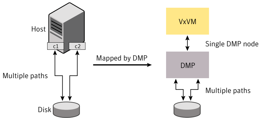
Figure 3-1 How DMP represents multiple physical paths to a disk as one node
