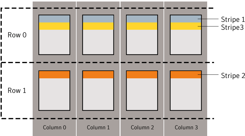
Figure 1-21 Traditional RAID-5 array
