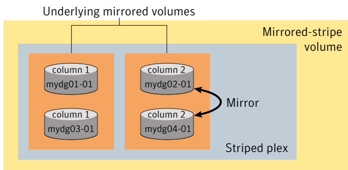
Figure 7-2 Example of using ordered allocation to create a striped-mirror volume
