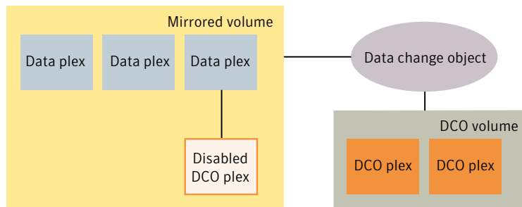
Figure 1-33 Mirrored volume after completion of a snapstart operation
