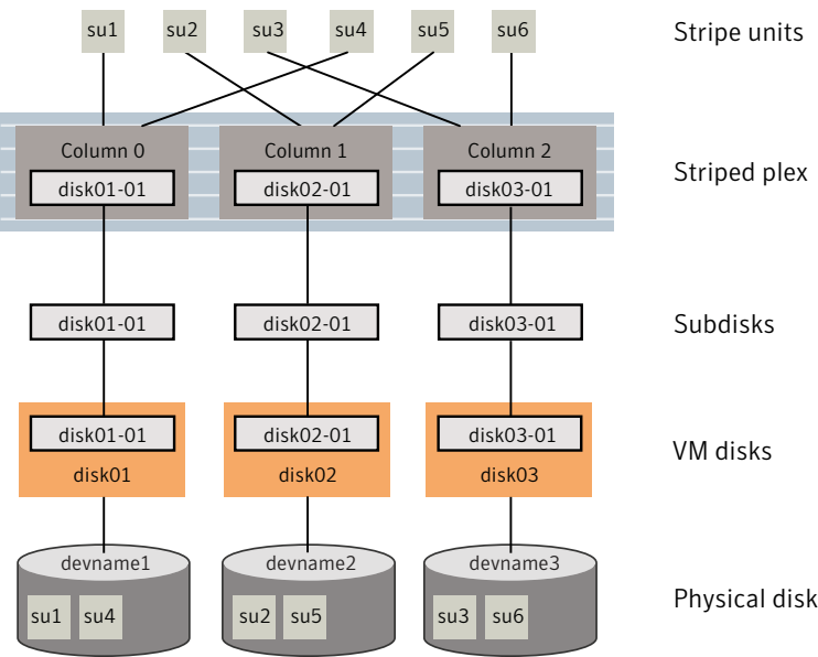
Figure 1-15 Example of a striped plex with one subdisk per column
