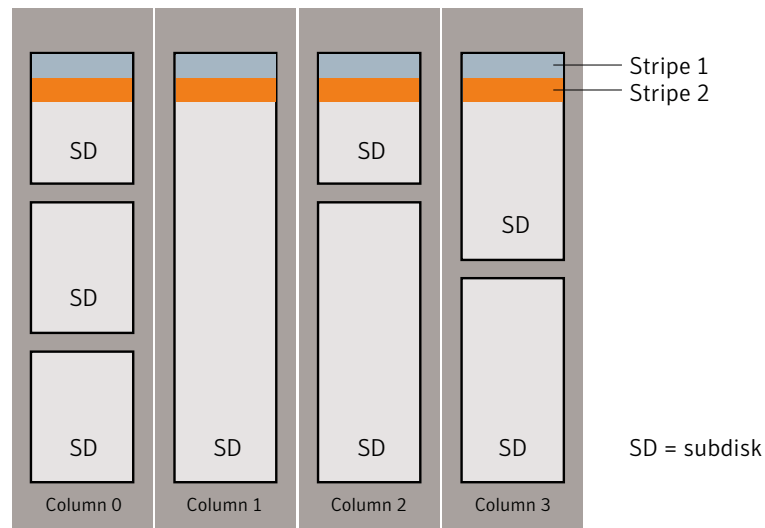
Figure 1-22 Veritas Volume Manager RAID-5 array
