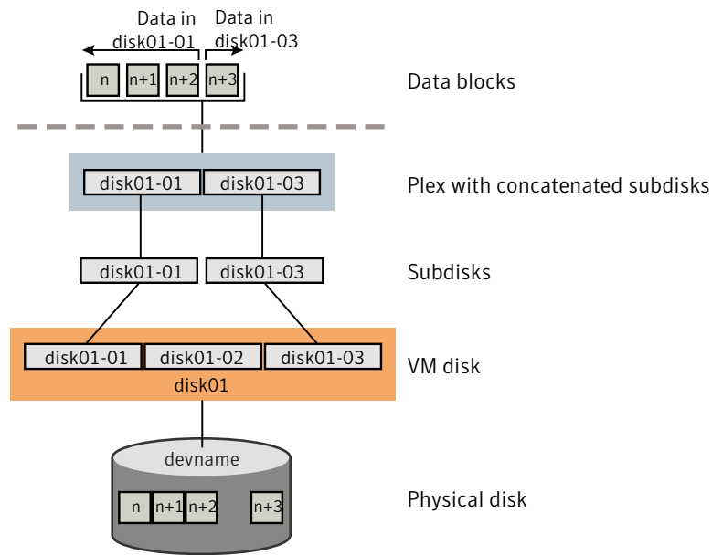
Figure 1-12 Example of concatenation
