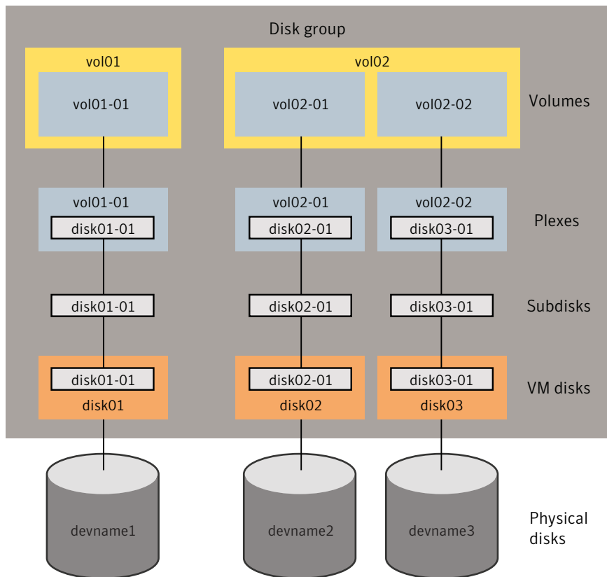
Figure 1-5 Connection between objects in VxVM
