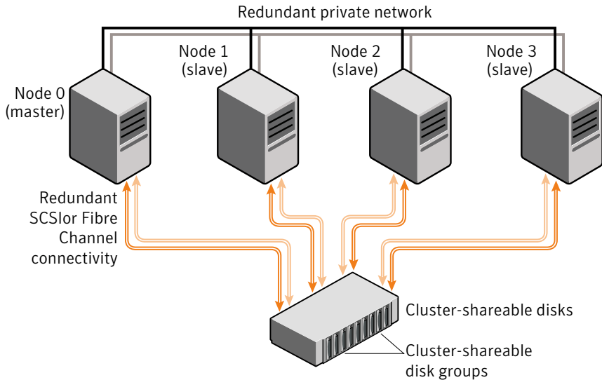
Figure 13-1 Example of a 4-node cluster
