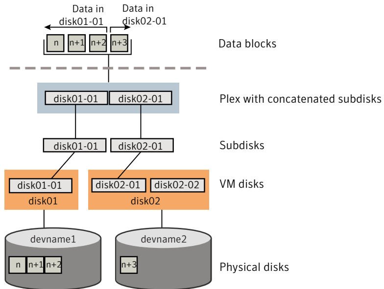
Figure 1-13 Example of spanning
