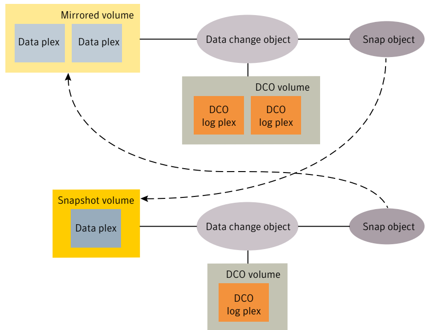
Figure 1-34 Mirrored volume and snapshot volume after completion of a snapshot operation
