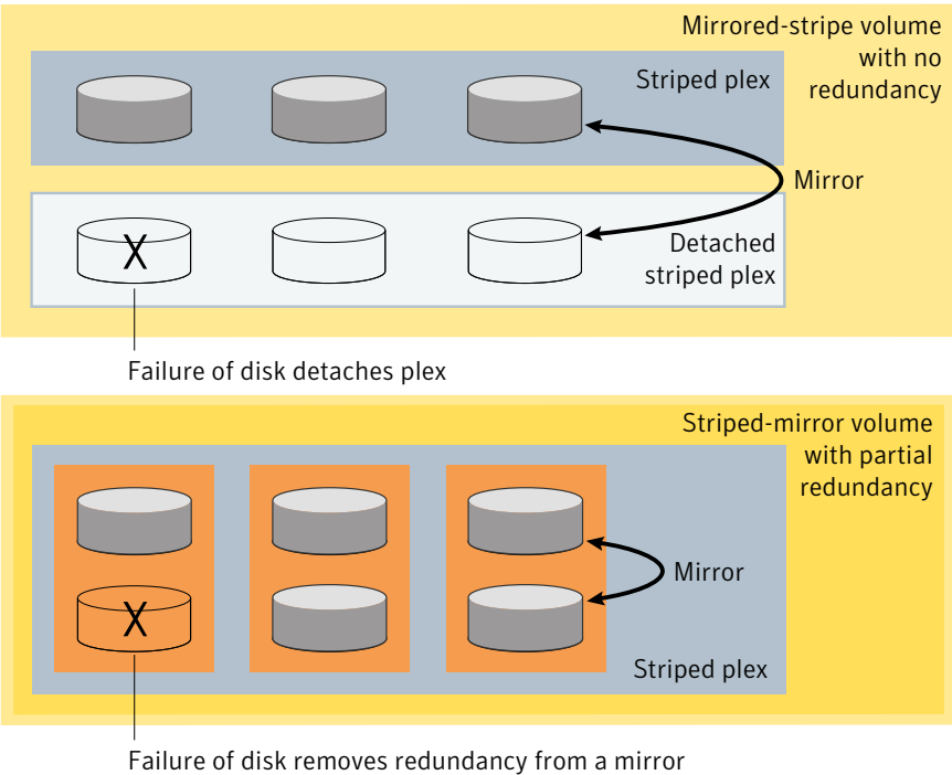
Figure 1-19 How the failure of a single disk affects mirrored-stripe and striped-mirror volumes
