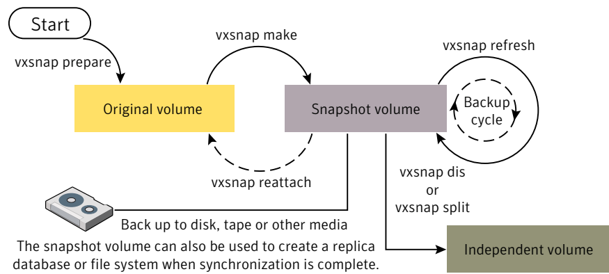
Figure 9-2 Full-sized instant snapshot creation and usage in a backup cycle
