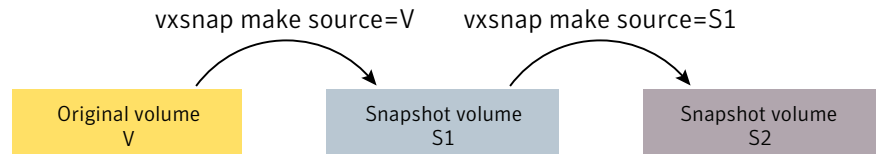
Figure 9-5 Creating a snapshot of a snapshot
