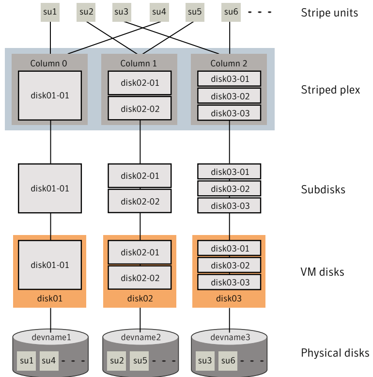
Figure 1-16 Example of a striped plex with concatenated subdisks per column
