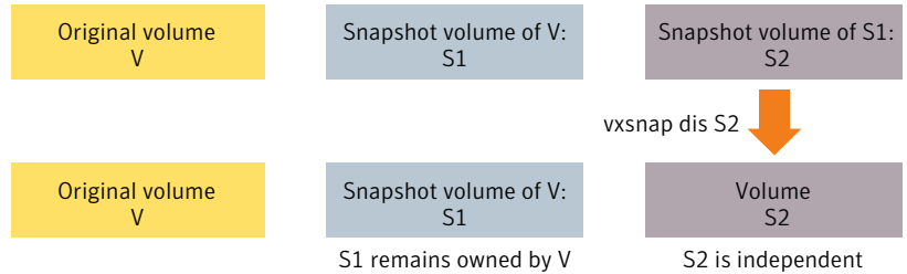
Figure 9-7 Dissociating a snapshot volume
