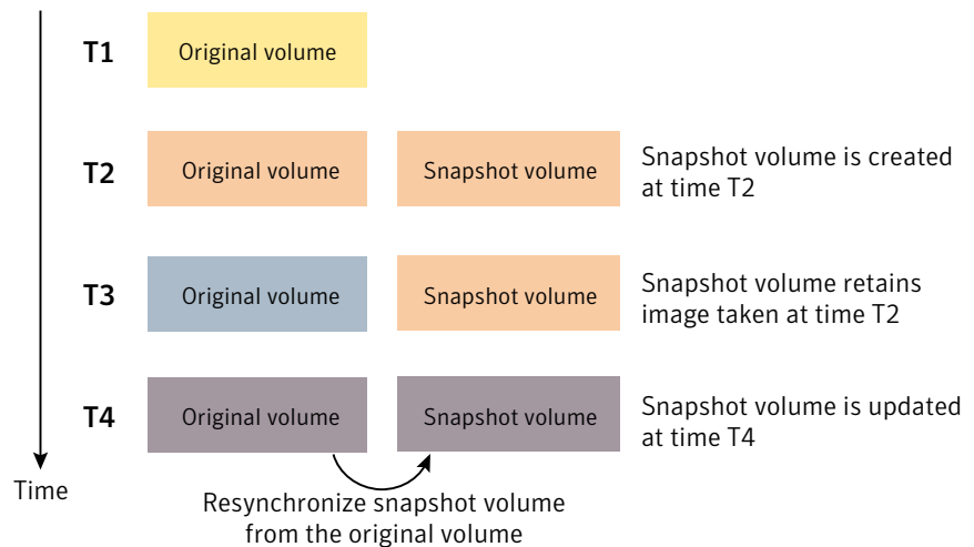
Figure 1-31 Volume snapshot as a point-in-time image of a volume
