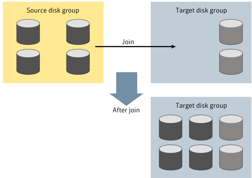
Figure 4-6 Disk group join operation
