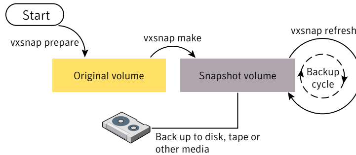
Figure 9-3 Space-optimized instant snapshot creation and usage in a backup cycle
