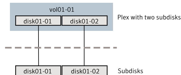
Figure 1-9 Example of a plex with two subdisks
