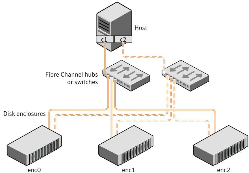
Figure 1-4 Example HA configuration using multiple hubs or switches to provide redundant loop access
