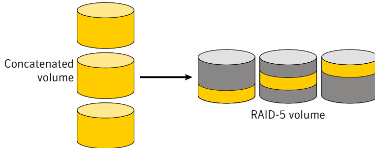
Figure 1-28 Example of relayout of a concatenated volume to a RAID-5 volume
