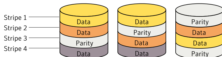
Figure 1-20 Parity locations in a RAID-5 model
