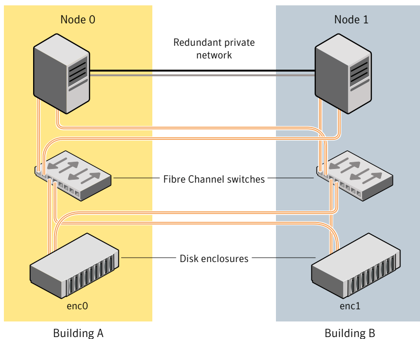
Figure 4-1 Typical arrangement of a 2-node campus cluster
