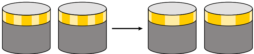
Figure 1-30 Example of increasing the stripe width for the columns in a volume
