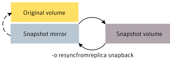
Figure 9-9 Resynchronizing an original volume from a snapshot
