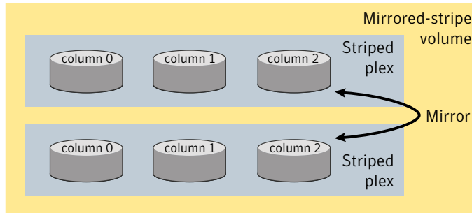
Figure 1-17 Mirrored-stripe volume laid out on six disks
