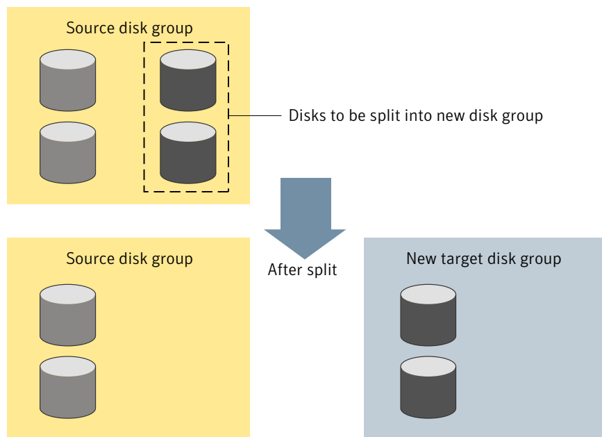
Figure 4-5 Disk group split operation
