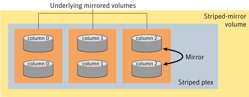
Figure 1-18 Striped-mirror volume laid out on six disks
