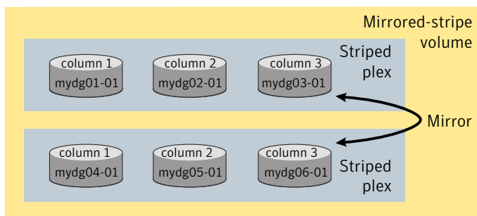
Figure 7-1 Example of using ordered allocation to create a mirrored-stripe volume
