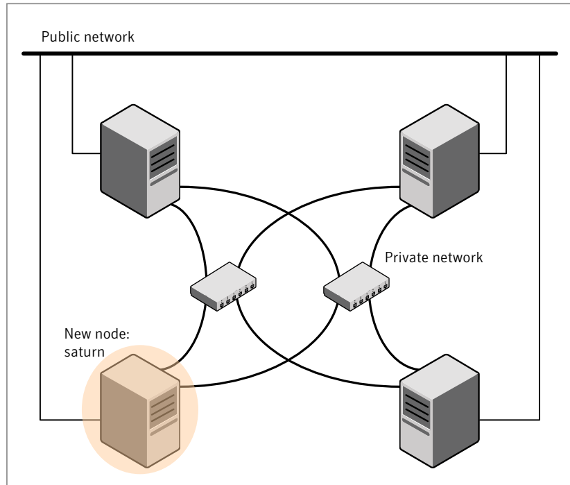
Figure 7-1 Adding a node to a three-node cluster using two independent hubs
