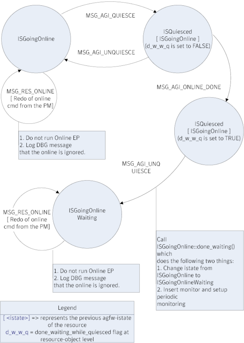
Quiescing and unquiescing of a resource in GoingOnline state
