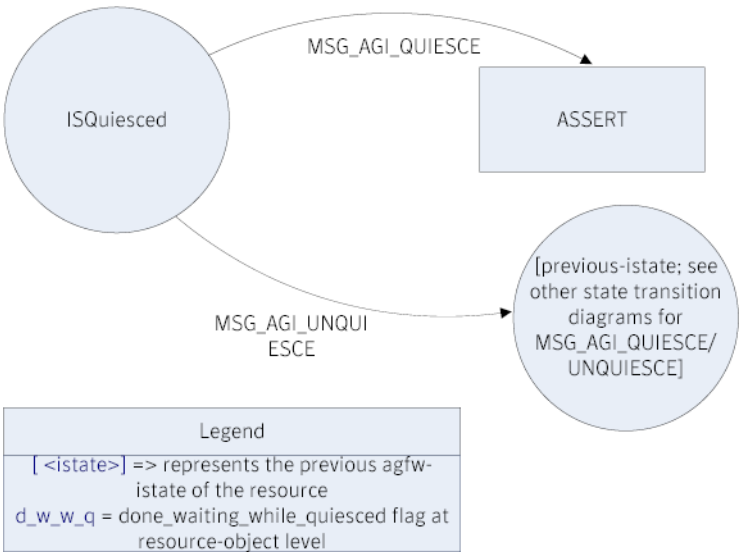
Quiescing and unquiescing of a resource in Quiesced state
