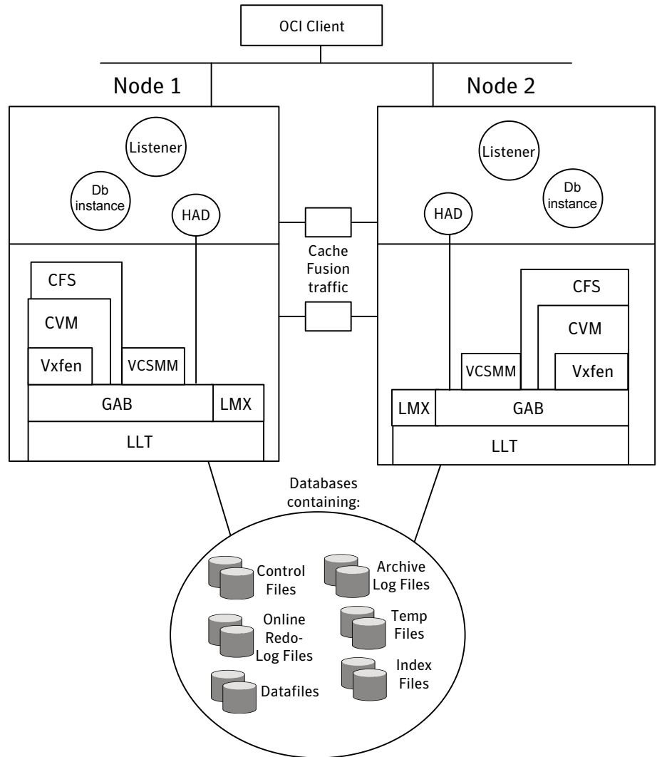
Figure 1-2 SF Oracle RAC architecture
