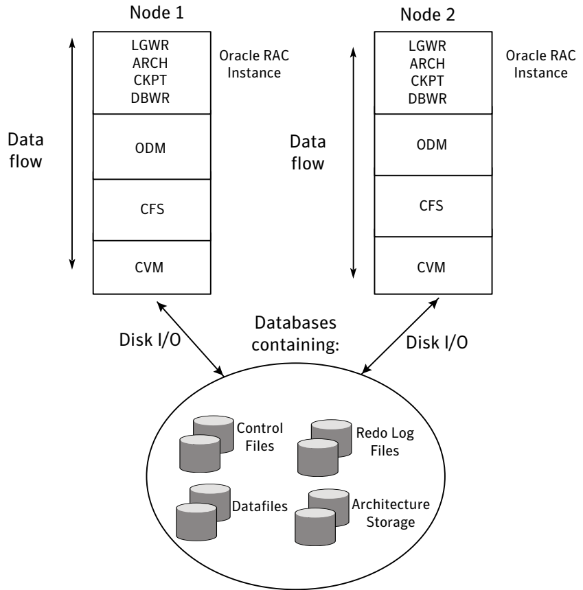
Figure 1-3 Data stack
