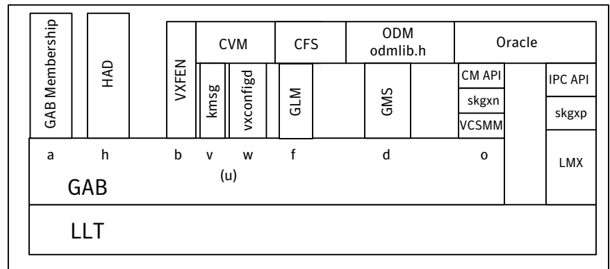
Figure 1-6 Low-level communication
