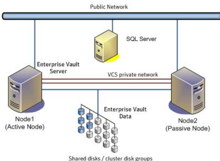
Figure 4-1 Active-Passive configuration
