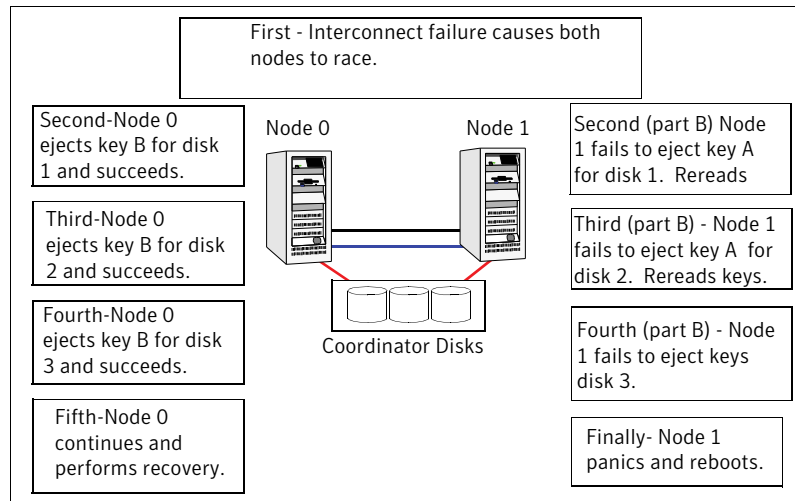
Figure 4-1 Preexisting network partition (split-brain)
