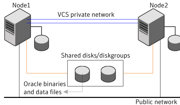
Figure 1-1 Oracle binaries and data on shared disks
