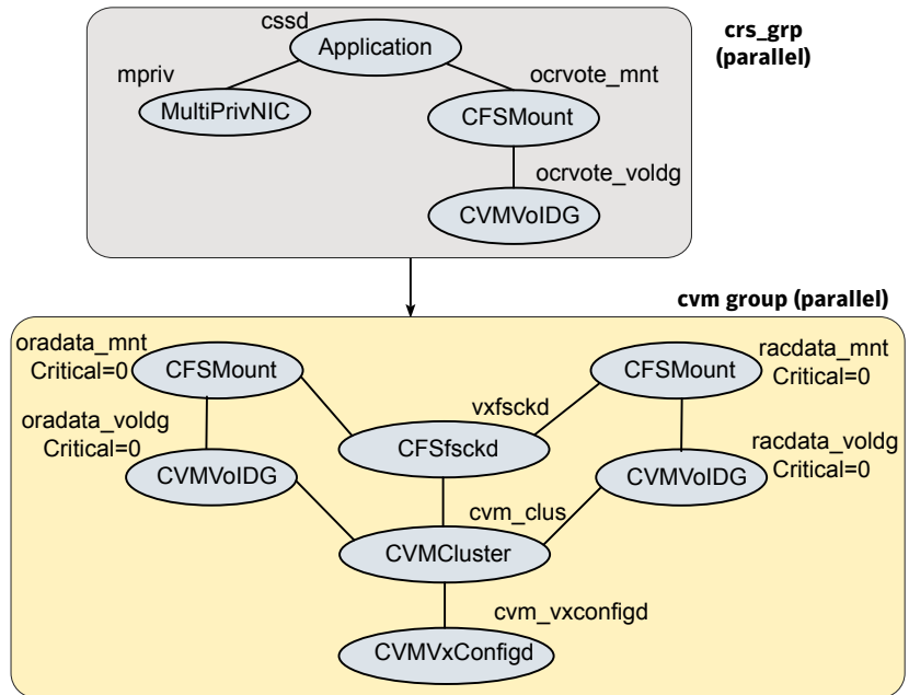
Figure 20-5 Service group configuration without the VCS Oracle agent (multiple databases)
