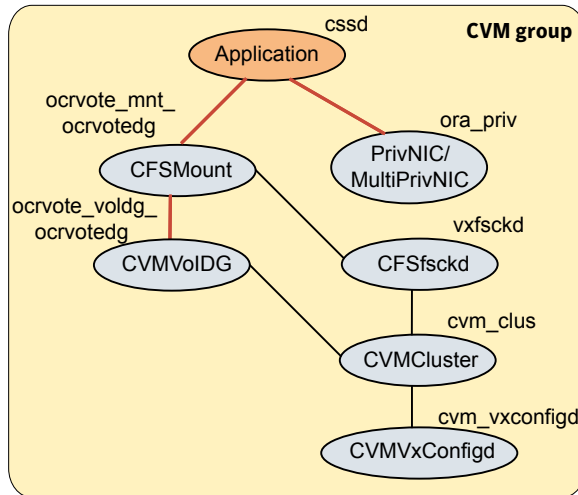
Figure 20-1 CSSD configuration by SF Oracle RAC installer
