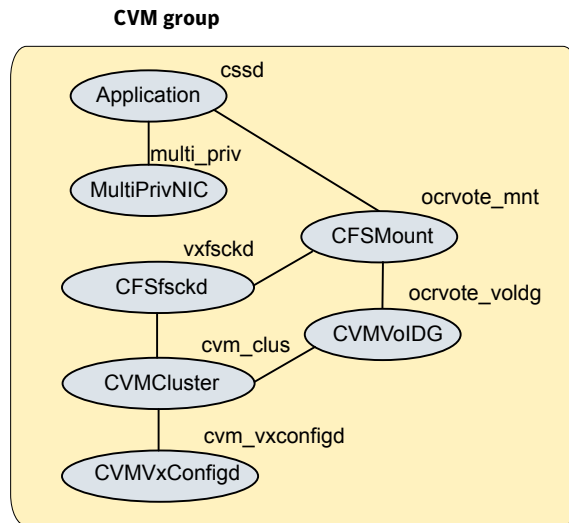
Figure 20-4 Service group configuration without VCS Oracle agent (single database)
