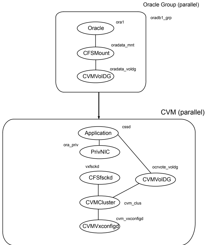
Figure 32-1 Illustration of dependencies before modification for replication
