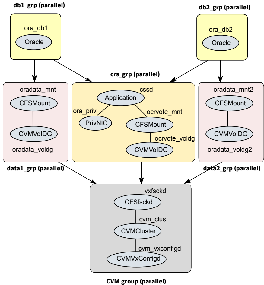
Figure 20-3 Service group configuration with the VCS Oracle agent (alternate configuration)
