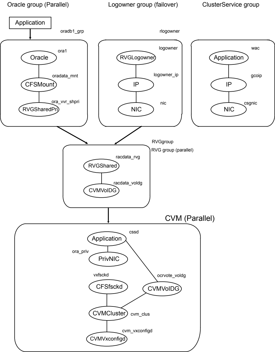
Figure 32-2 Illustration of dependencies after modification for replication for Oracle RAC
