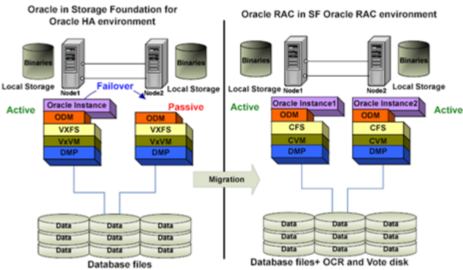
Figure 16-1 Migration from Storage Foundation for Oracle HA to SF Oracle RAC
