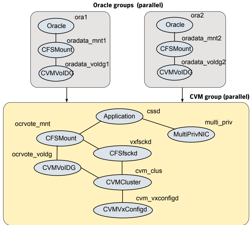
Figure 20-2 Service group configuration with the VCS Oracle agent
