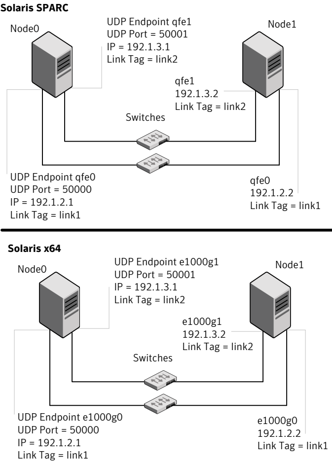
Figure L-1 A typical configuration of direct-attached links that use LLT over UDP
