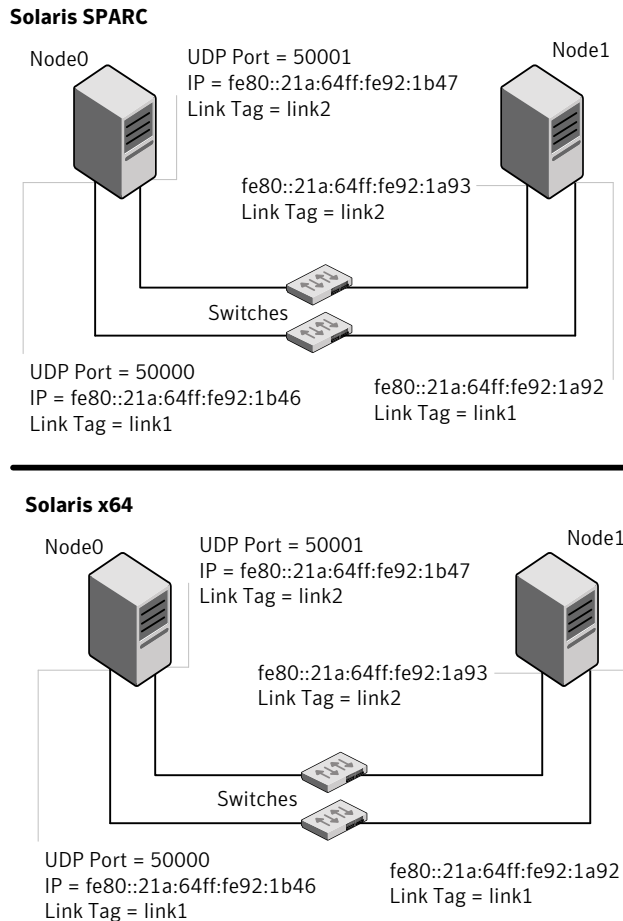
Figure M-1 A typical configuration of direct-attached links that use LLT over UDP
