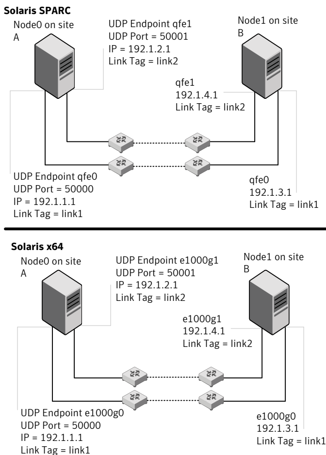
Figure L-2 A typical configuration of links crossing an IP router
