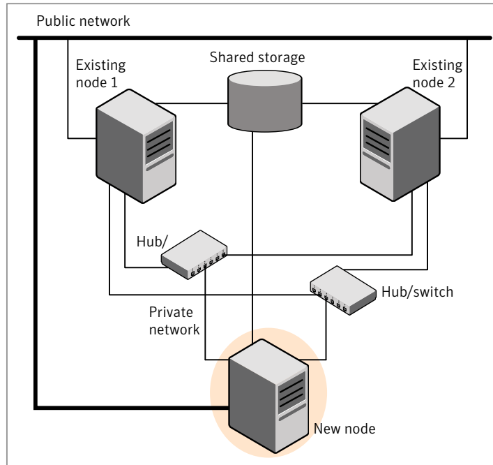
Figure 11-1 Adding a node to a two-node cluster using two switches
