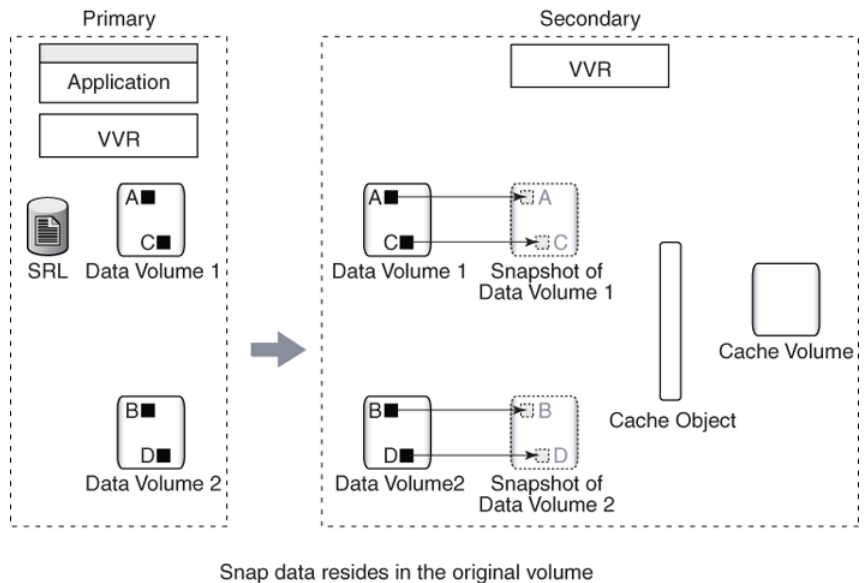
Figure 2-11 Example 1—How VVR creates instant space-optimized snapshots
