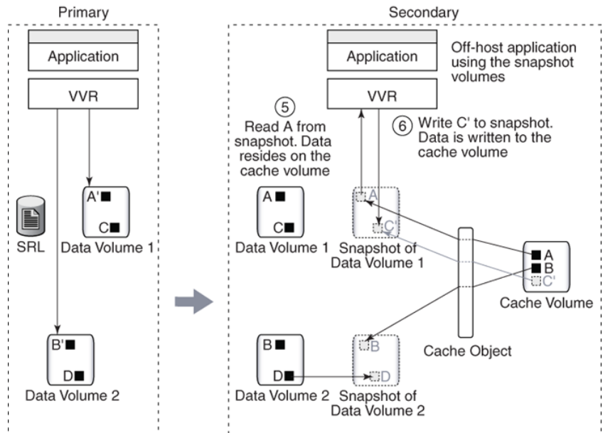
Figure 2-13 Example 3—How VVR reads the changed block from the cache object
