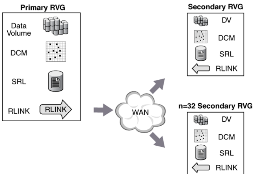
Figure 1-2 Sample configuration to illustrate the VVR components
