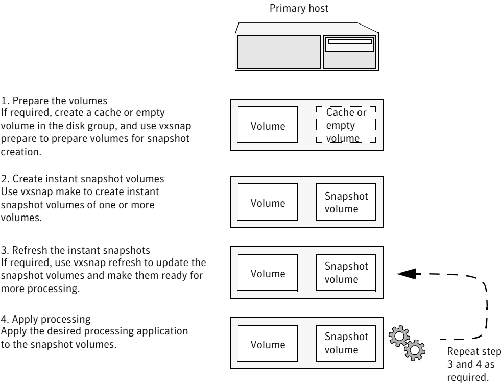
Figure 15-1 Using snapshots and FastResync to implement point-in-time copy solutions on a primary host
