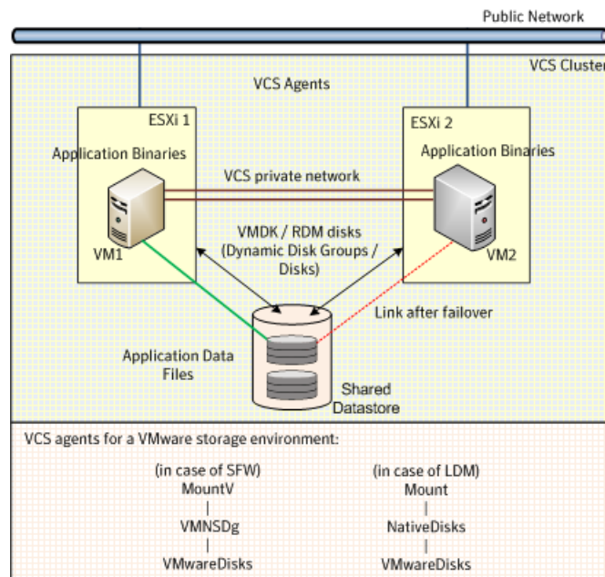
Figure 1-1 Typical services, processes, and mount points cluster configuration in a VMware virtual environment
