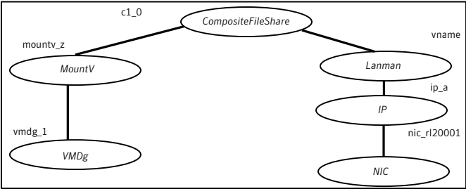
Figure 4-2 CompositeFileShare service group dependency graph
