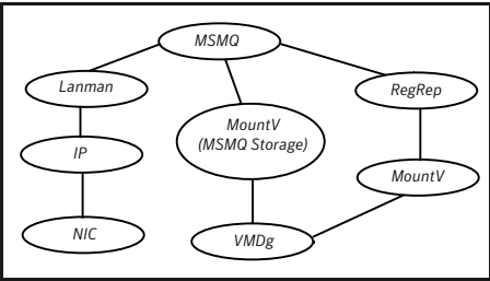
Figure 6-3 MSMQ agent dependency graph
