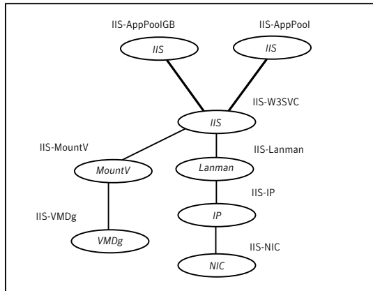
Figure 6-2 IIS service group dependency graph
