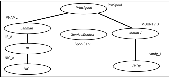
Figure 5-1 PrintSpool service group dependency graph
