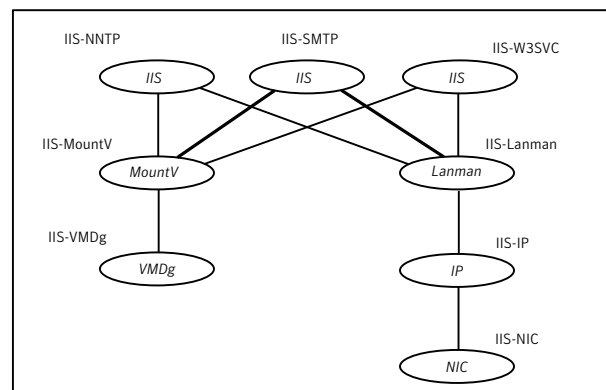
Figure 6-1 IIS service group dependency graph
