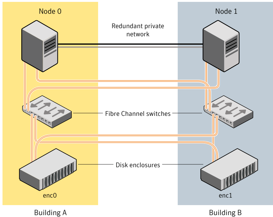
Figure 31-5 Typical arrangement of a 2-node campus cluster
