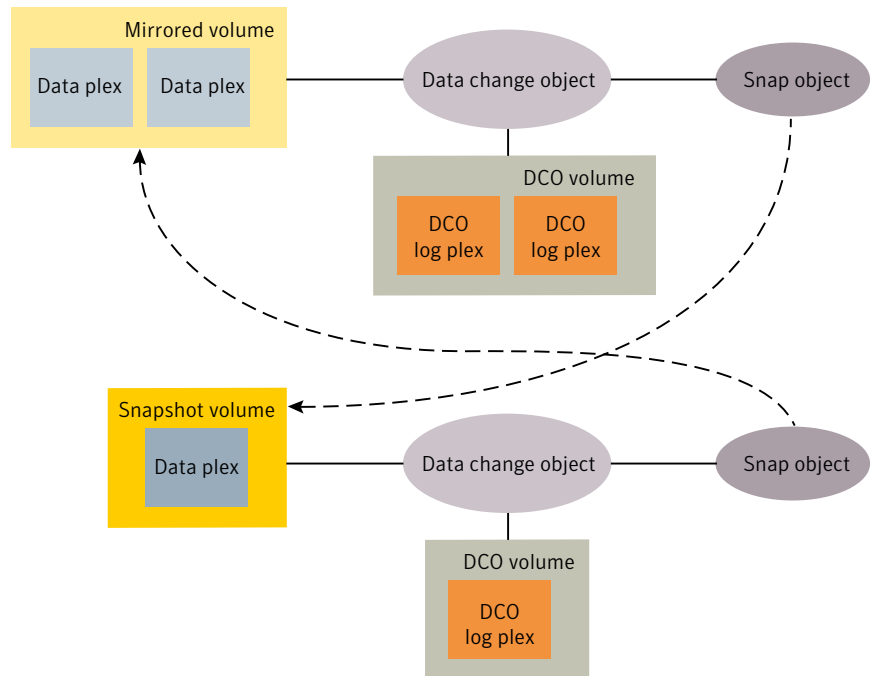
Figure 3-26 Mirrored volume and snapshot volume after completion of a snapshot operation
