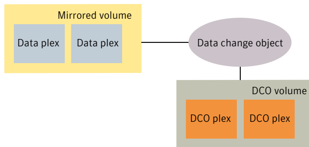
Figure 3-24 Mirrored volume with persistent FastResync enabled
