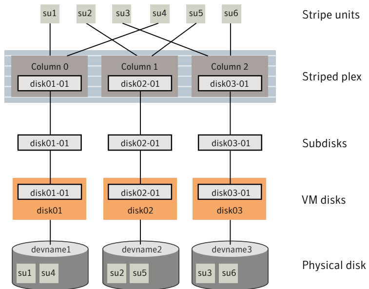
Figure 3-7 Example of a striped plex with one subdisk per column
