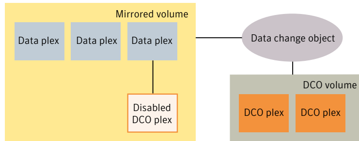
Figure 3-25 Mirrored volume after completion of a snapstart operation
