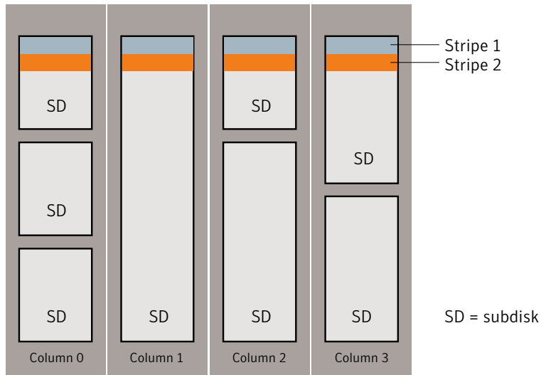
Figure 3-14 Veritas Volume Manager RAID-5 array
