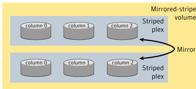
Figure 3-9 Mirrored-stripe volume laid out on six disks
