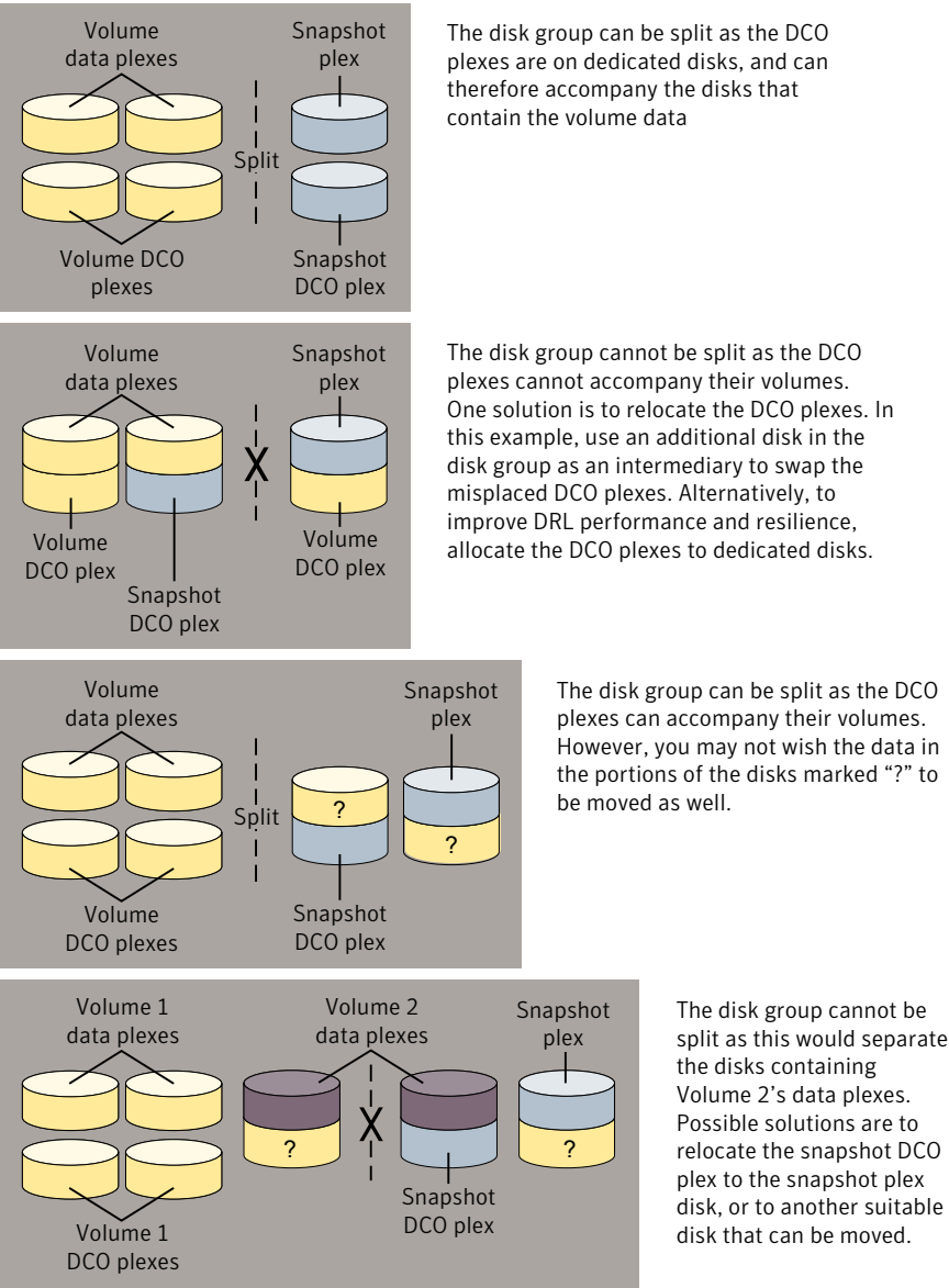
Figure 31-4 Examples of disk groups that can and cannot be split
