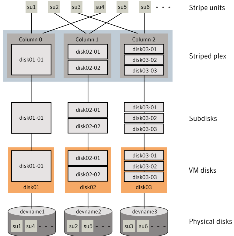
Figure 3-8 Example of a striped plex with concatenated subdisks per column
