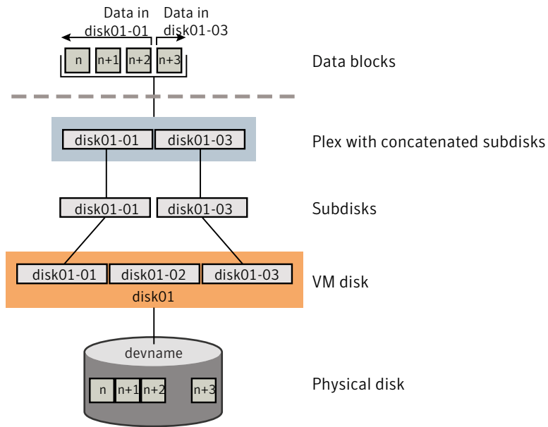
Figure 3-4 Example of concatenation
