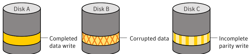
Figure 3-16 Incomplete write to a RAID-5 volume
