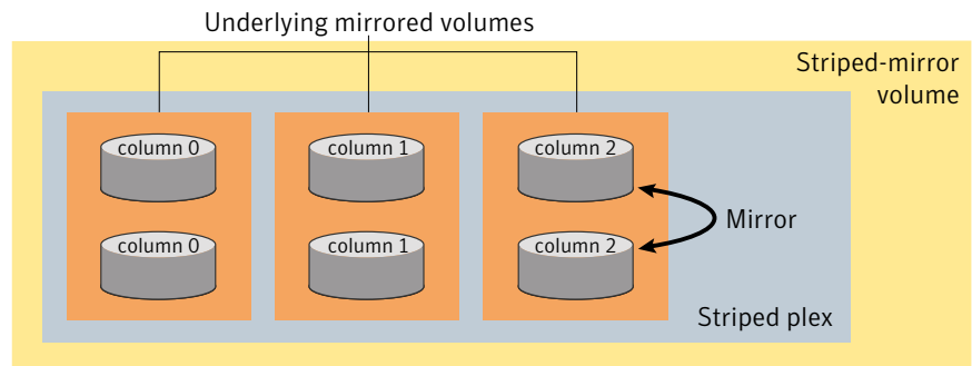
Figure 3-10 Striped-mirror volume laid out on six disks
