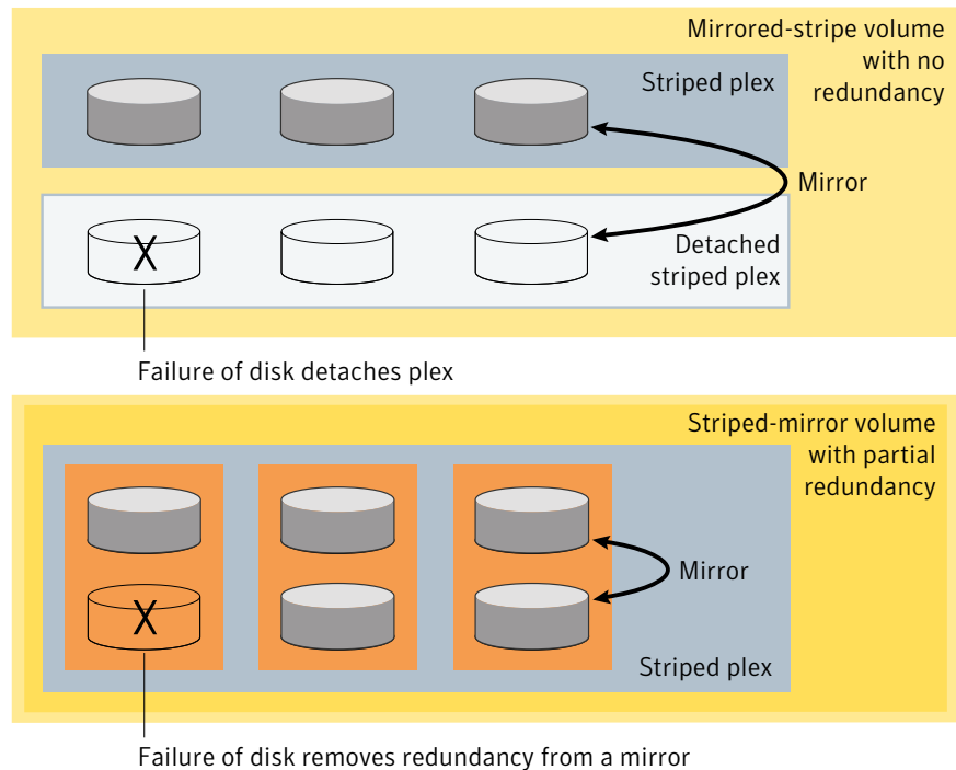
Figure 3-11 How the failure of a single disk affects mirrored-stripe and striped-mirror volumes
