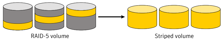
Figure 3-19 Example of relayout of a RAID-5 volume to a striped volume
