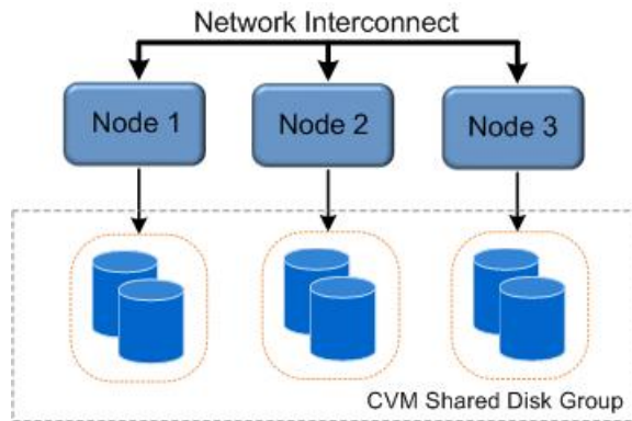
Figure 11-1 Flexible Storage Sharing Environment
