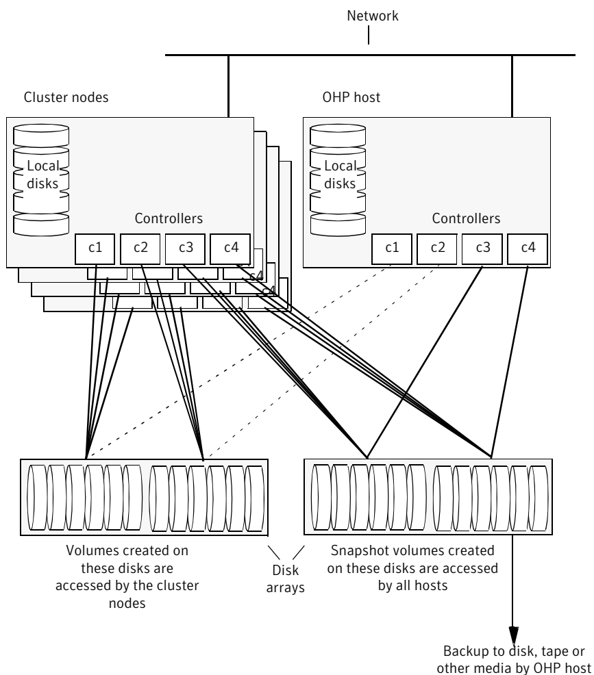
Figure 5-3 System configuration for off-host file system backup scenarios
