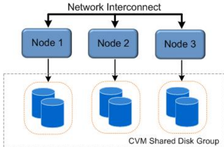
Figure 6-11 Flexible Storage Sharing Environment
