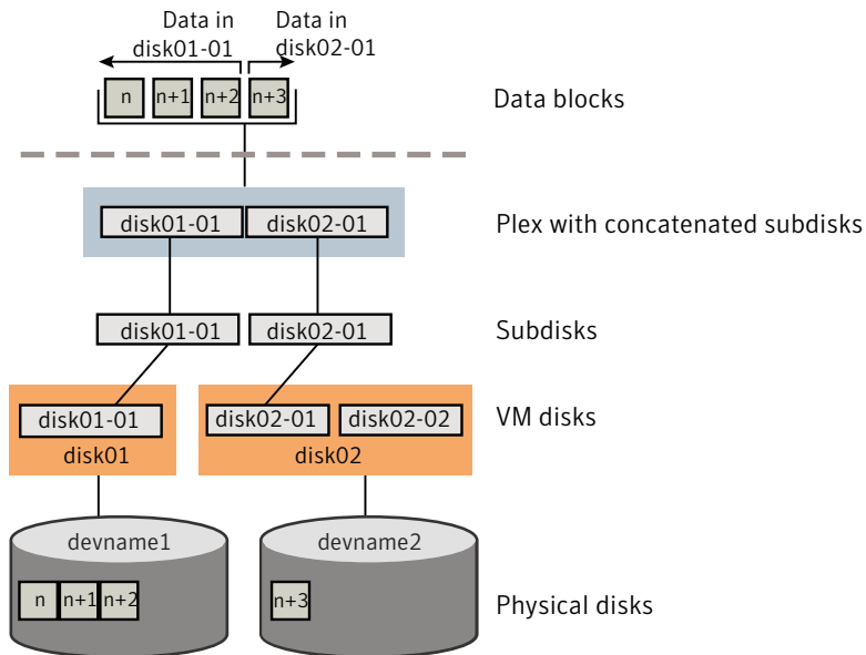
Figure 3-6 Example of spanning
