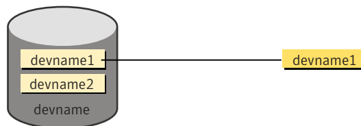
Figure 3-2 Partition example
