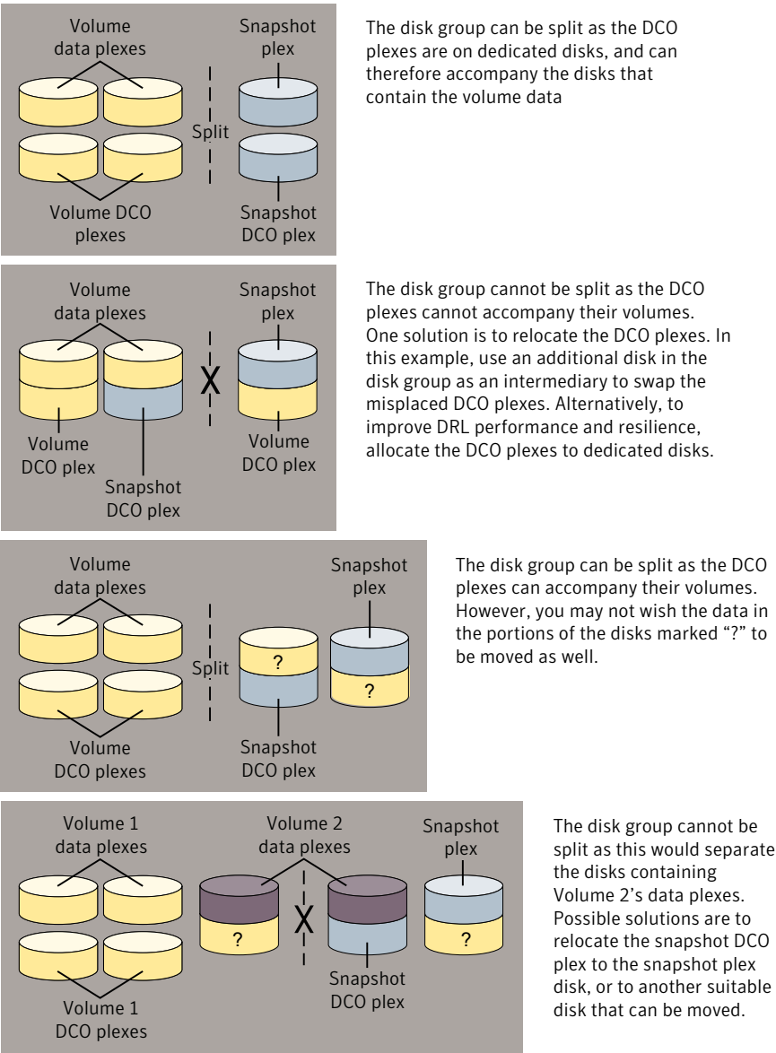
Figure 30-4 Examples of disk groups that can and cannot be split
