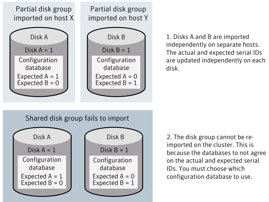
Figure 30-7 Example of a true serial split brain condition that cannot be resolved automatically
