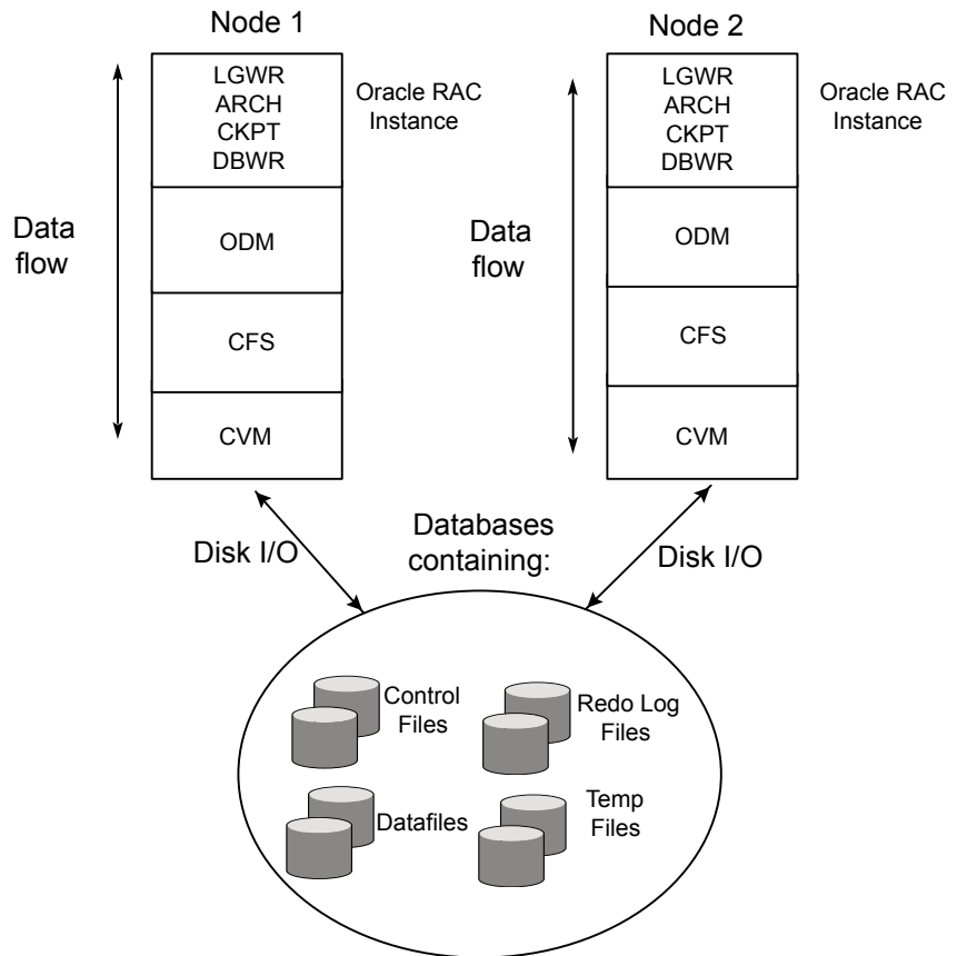
Figure 1-3 Data stack
