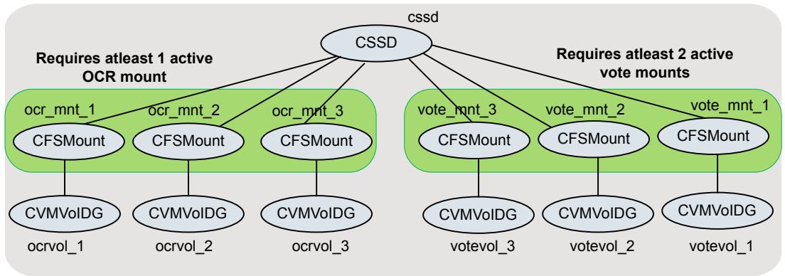
Figure 10-1 Atleast resource dependency for OCR and voting disks
