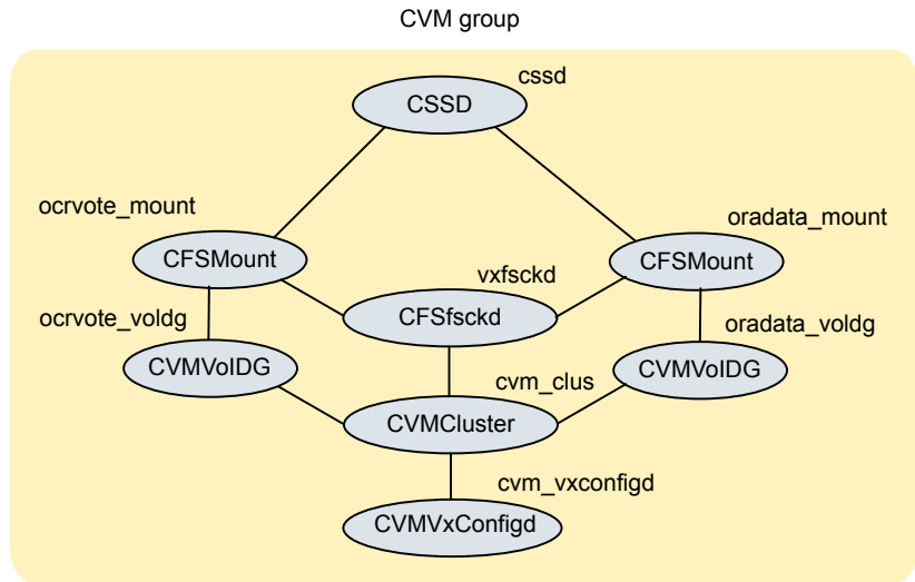
Figure 13-5 Service group configuration without VCS Oracle agent (single database)
