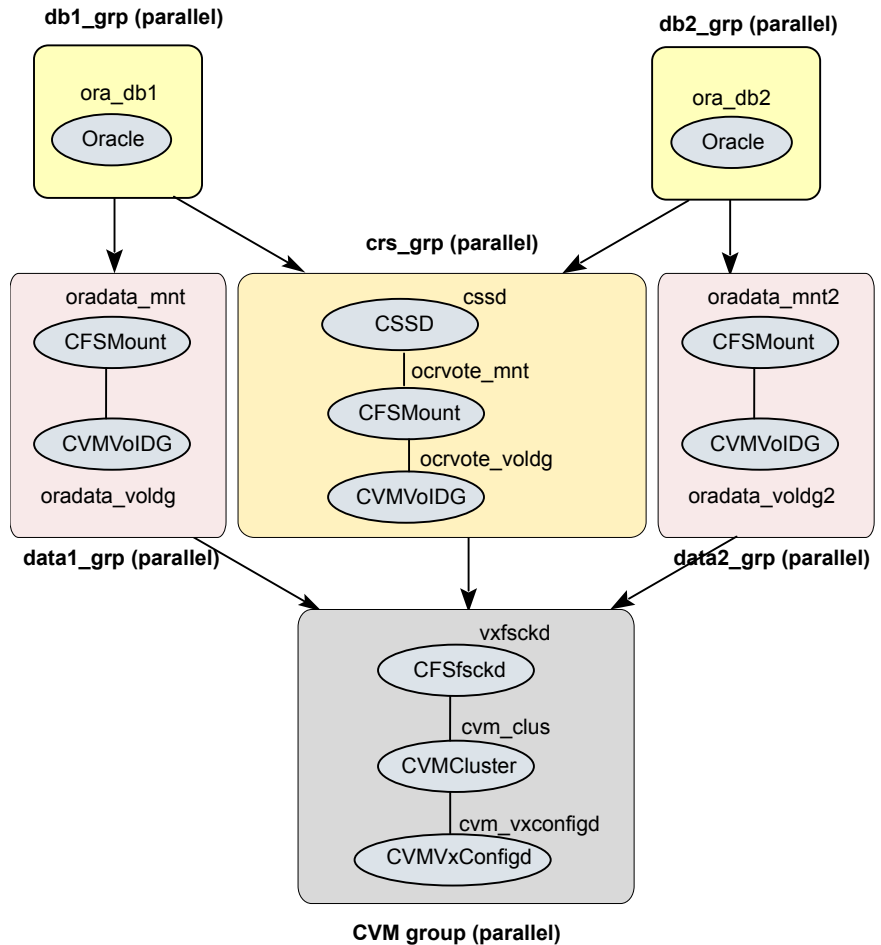
Figure 13-4 Service group configuration with the VCS Oracle agent (alternate configuration)
