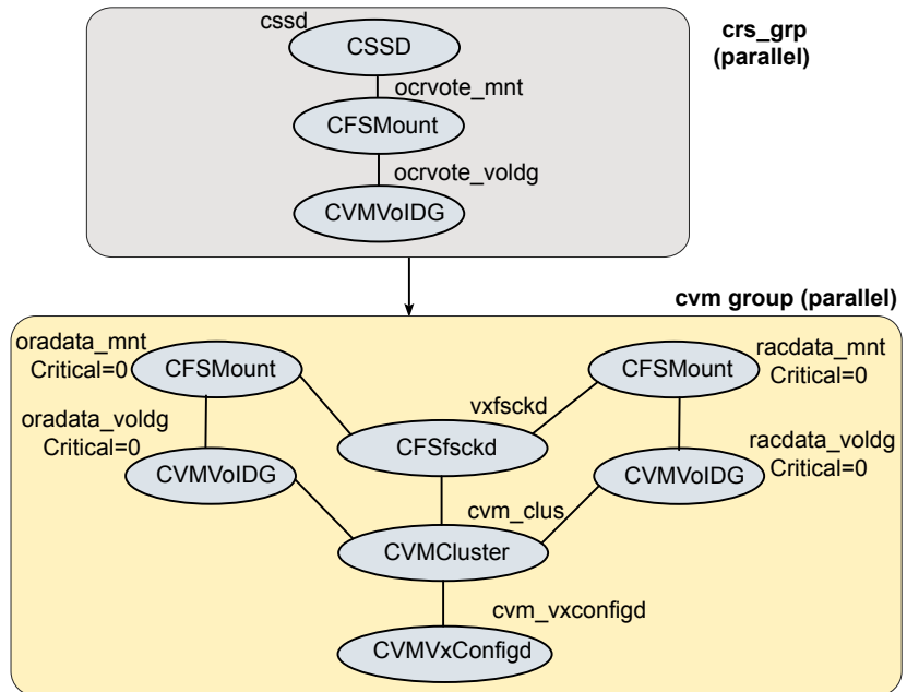
Figure 13-6 Service group configuration without the VCS Oracle agent (multiple databases)
