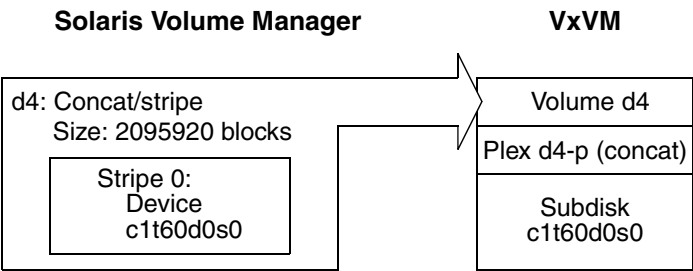
Figure C-1 Single Solaris Volume Manager partition encapsulated in a concat/stripe Solaris Volume Manager object
