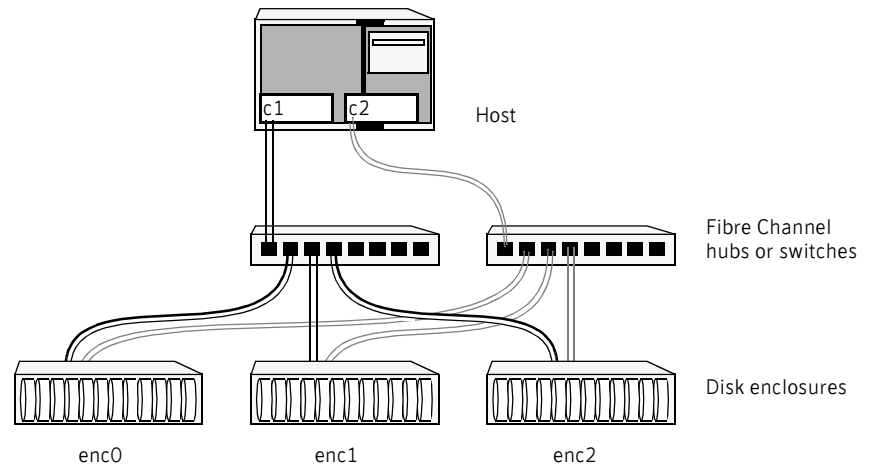
Figure 1-5 Example HA configuration using multiple hubs or switches to provide redundant loop access
