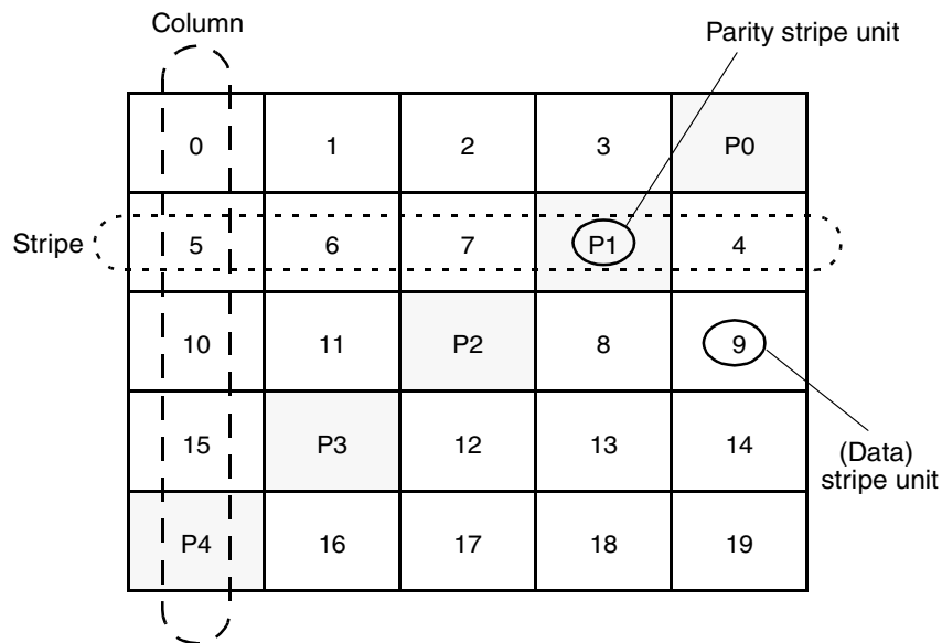
Figure 1-24 Left-symmetric layout
