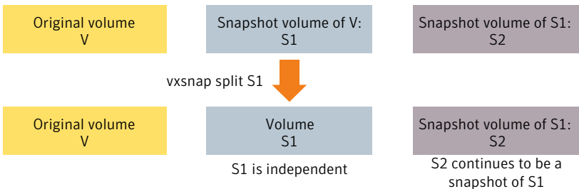
Figure 9-8 Splitting snapshots
