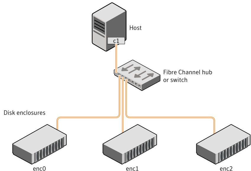
Figure 1-3 Example configuration for disk enclosures connected via a fibre channel hub or switch
