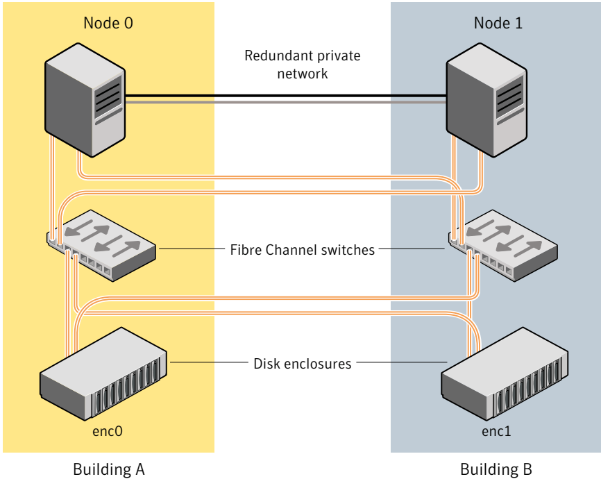
Figure 4-1 Typical arrangement of a 2-node campus cluster
