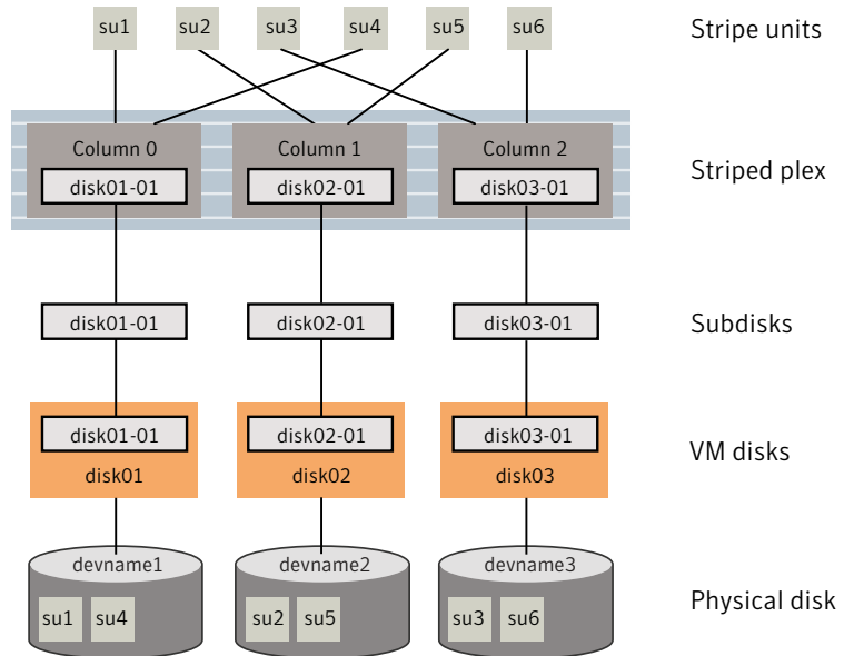
Figure 1-15 Example of a striped plex with one subdisk per column
