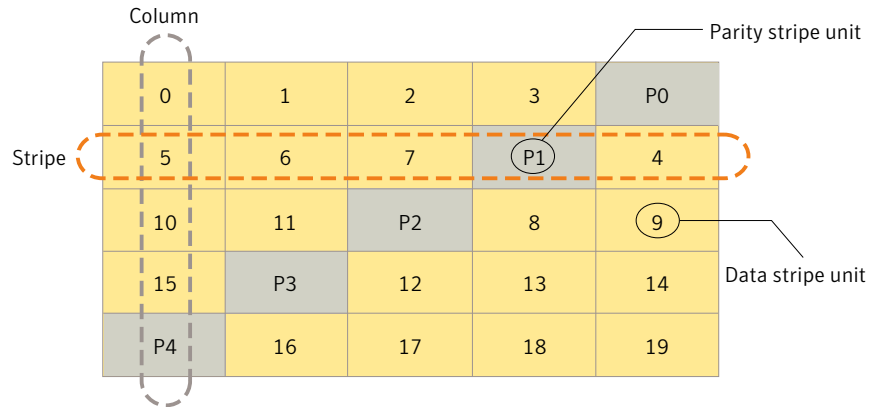
Figure 1-23 Left-symmetric parity layout
