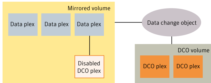
Figure 1-33 Mirrored volume after completion of a snapstart operation
