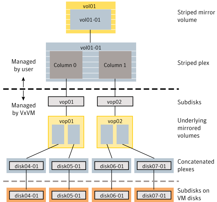
Figure 1-25 Example of a striped-mirror layered volume
