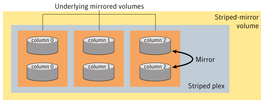
Figure 1-18 Striped-mirror volume laid out on six disks
